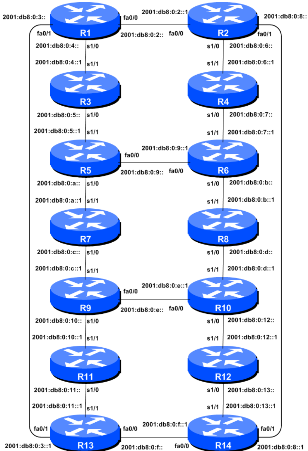
Figure 1 – Addressing scheme for Modules 1 to 5
